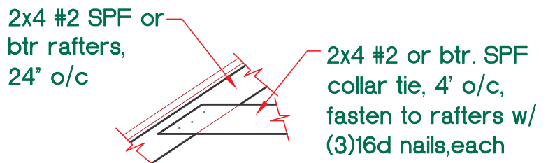
Detail B-B/4 Scale \frac{3}{4} " = 1'-0"
