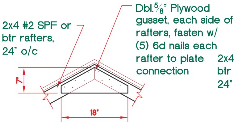
Detail A-A/4 Scale \frac{3}{4} " = 1'-0"
